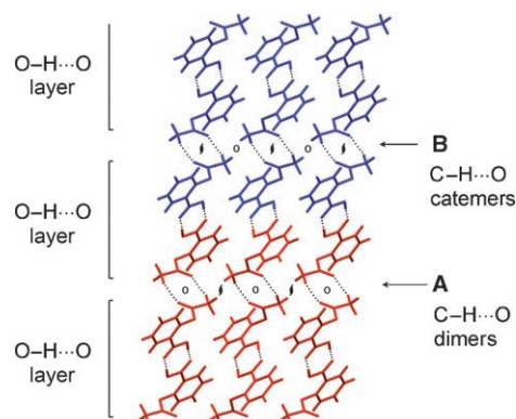
Figure 1. Illustration of the two interlayer arrangements within a representative aspirin crystal. Arrangement A , comprising centrosymmetric C–H...O dimers, exists between the layers that are colored red. Arrangement B , comprising C–H...O catemers extending along 2_1 screw axes, exists between the layers that are colored blue. The change in color within the central layer is for illustration only; all O–H...O hydrogen-bonded layers are identical.
