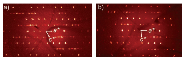
Figure 2. Reconstructed ( h-k ) precession photographs for crystals 1a and 2 . a) Crystal 1a exhibits sharp Bragg reflections corresponding to the form II lattice (reciprocal lattice vectors shown), broader maxima halfway between these reflections in the odd l rows, and diffuse streaks along a^* . This indicates extended form II domains, smaller domains of form I, and regions in which there is a disordered distribution. b) For crystal 2 , the most intense Bragg reflections correspond to the form I lattice (reciprocal lattice vectors shown), and Bragg reflections of comparable profile exist for the form II lattice. This indicates a relatively more ordered structure than in 1a (a) with extended form I and form II domains.
