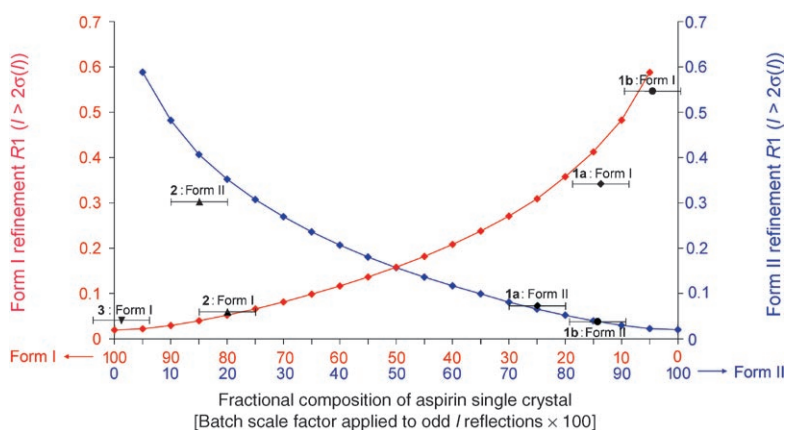
Figure 3. Correlation between total domain ratio and expected crystallographic R1 value, obtained for conventional refinement against all F^2 data. The correlation is derived from experimental data for crystal 3 (see the Supporting Information for full details). The red and blue curves refer to standard data reduction and refinement on the basis of the form I and form II structures, respectively, for an aspirin crystal with domain ratio indicated by the horizontal axis. The experimental points correspond to the R values obtained for the crystals listed in Table 1. For these, the composition estimate is taken from the batch scale factor refinement, with error bars indicating \pm 5\% composition. For example, conventional refinement of crystal 1a as form II gives R1 = 0.071 . The separate batch scale factor refinement indicates 75% form II domains. The same crystal 1a refined conventionally as form I gives R1 = 0.344 , with the separate batch scale factor refinement indicating 15% form I domains.
